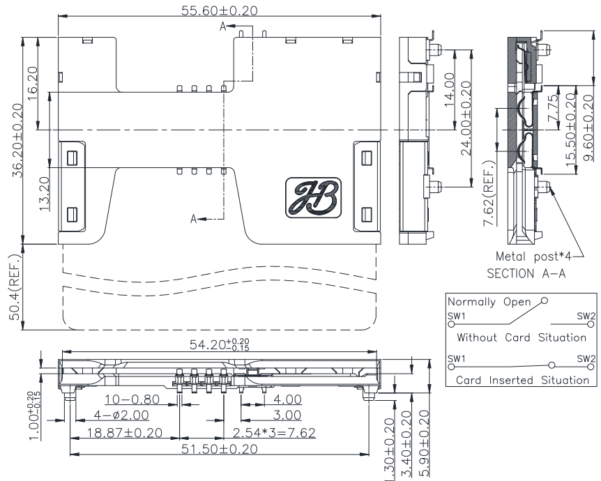
Unit: mm; Tolerances: ±0.15 mm Mechanical outline dimension
