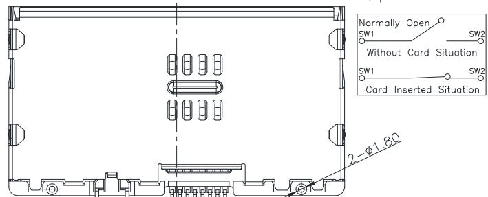
Unit: mm; Tolerances: ±0.15 mm Mechanical outline dimension
