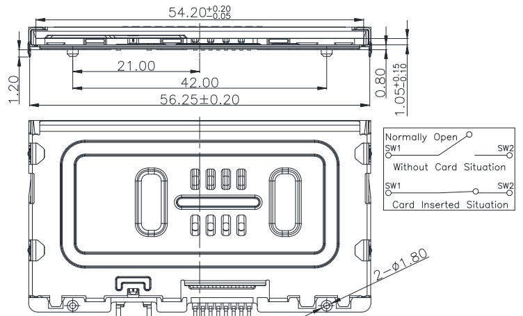
Unit: mm; Tolerances: ±0.15 mm Mechanical outline dimension
